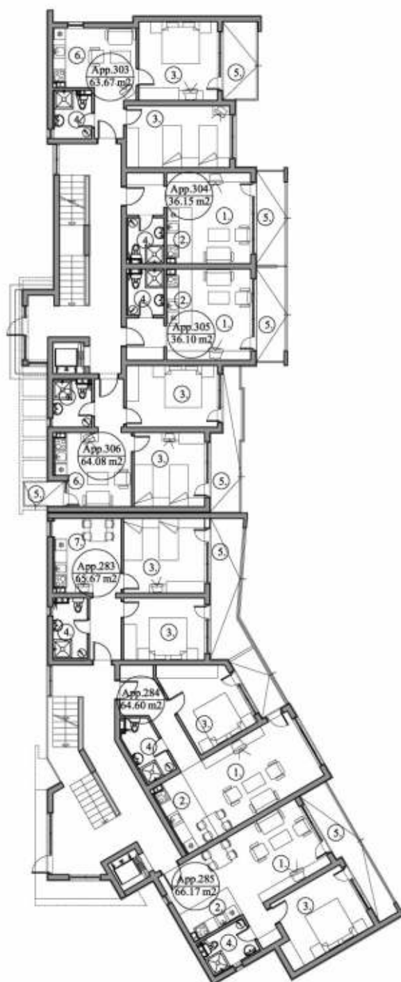
C6 SECOND FLOOR SCALE 1:200
